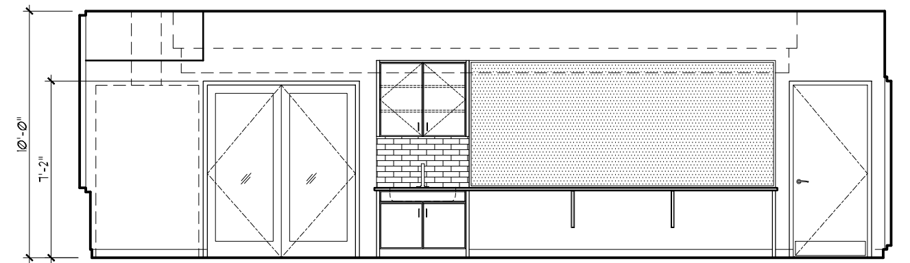
4 INTERIOR ELEVATION INNOVATION LAB #108 SCALE: 1/4"=1'-0"
