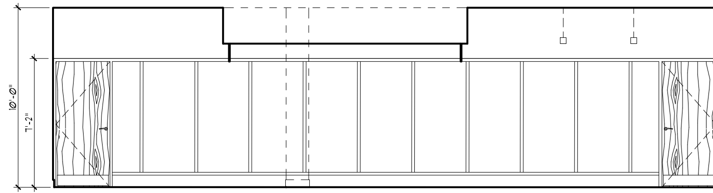
1 INTERIOR ELEVATION INNOVATION LAB #108 SCALE: 1/4"=1'-0"
