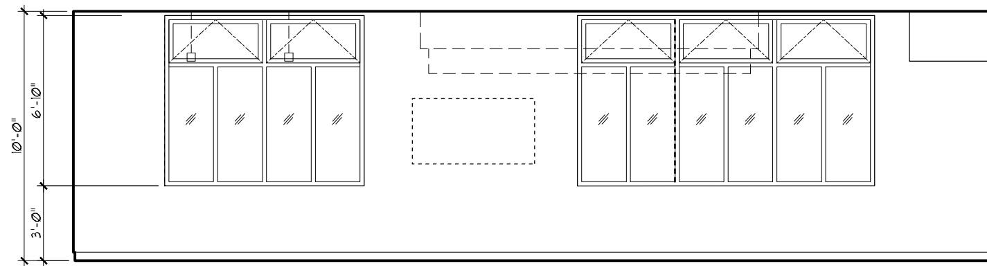
3 INTERIOR ELEVATION INNOVATION LAB #108 SCALE: 1/4"=1'-0"
